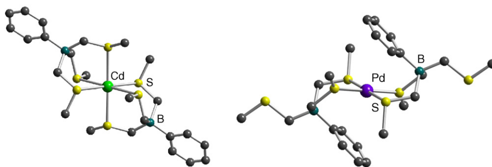
Fig. 3. Structures of [\text{PhTt}]_2\text{Cd} and [\text{PhTt}]_2\text{Pd} .
