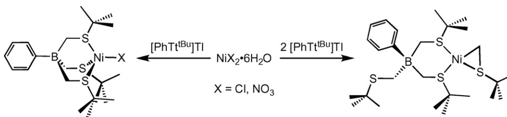
Scheme 2. Synthesis of [\text{PhTt}^{\text{tBu}}]\text{NiX} and [\kappa^2\text{-PhTt}^{\text{tBu}}]\text{Ni}(\text{CH}_2\text{S}^{\text{tBu}}) .
