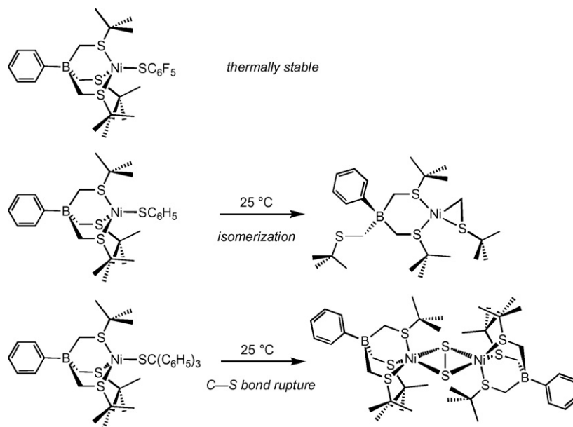
Scheme 4. Thermal reactivity of [\text{PhTt}^{\text{tBu}}]\text{Ni}(\text{SR}) .
