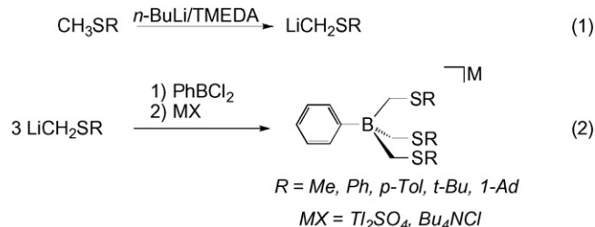
Scheme 1. Ligand synthesis.
