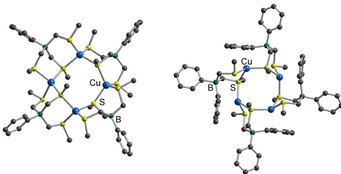
Fig. 4. [(\text{PhTt})\text{Cu}]_4 (left) and [(\text{Ph}_2\text{Bt})\text{Cu}]_4 (right).
