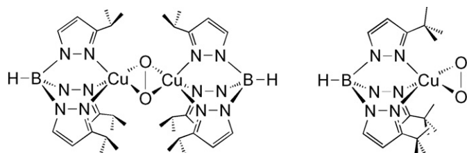
Fig. 1. Kitajima's [\text{Tp}^{\text{R}}]\text{Cu} peroxo (left) and superoxo (right) complexes.
