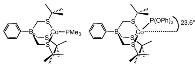
Fig. 8. Structures of Co(I) complexes as a function of phosphine: σ-donor phosphines reside on the three-fold axis, whereas π-acceptor ligands lead to a distorted geometry.
