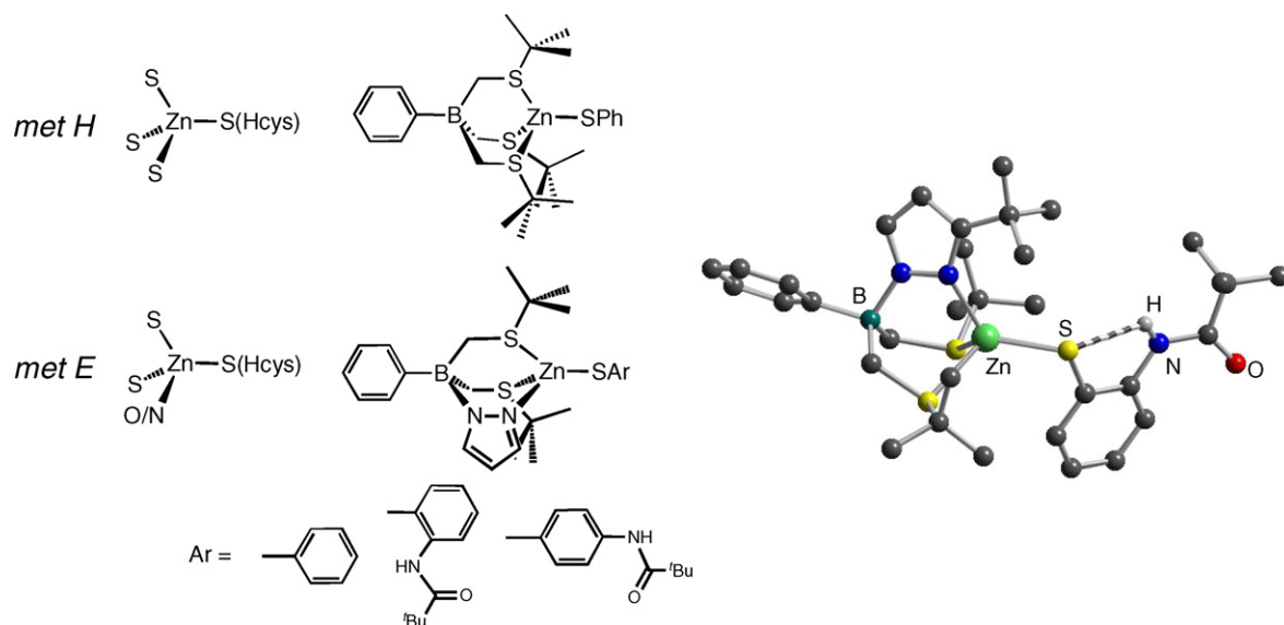
Fig. 7. Active site coordination environments and associated model complexes for the homocysteine (Hcys) ligated states of the zinc sites in the methionine synthases and structure of synthetic complex containing an internal S...H-N bond (right).
