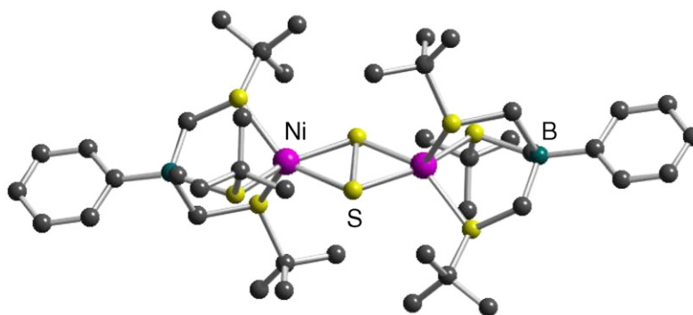
Fig. 9. Structure of [(\text{PhTt}^{\text{tBu}})\text{Ni}]_2(\mu\text{-}\eta^2\text{:}\eta^2\text{-S}_2) .
