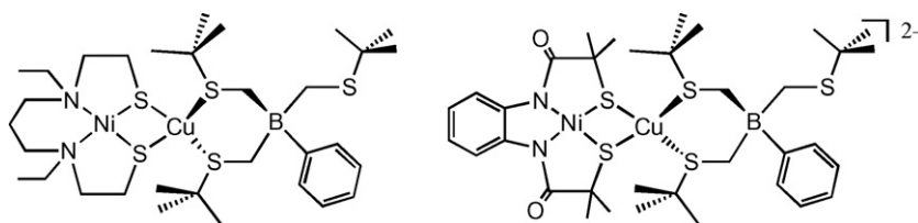
Fig. 5. Thiolate-bridged nickel–copper complexes, (\text{Et}_2\text{N}_2\text{S}_2)\text{NiCu}[\text{PhTt}^{\text{tBu}}] and [(\text{phmi})\text{NiCu}(\text{PhTt}^{\text{tBu}})]^{2-} .
