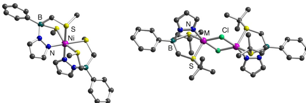
Fig. 6. \text{cis-}[\text{Ph}(\text{pz})\text{Bt}]_2\text{Ni} and [(\text{Ph}(\text{pz})\text{Bt})\text{M}]_2(\mu\text{-Cl})_2 ( \text{M} = \text{Co}, \text{Ni} ).
