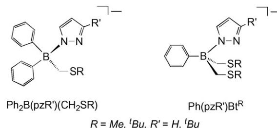
Fig. 2. [\text{SN}] and [\text{S}_2\text{N}] borate ligands.
